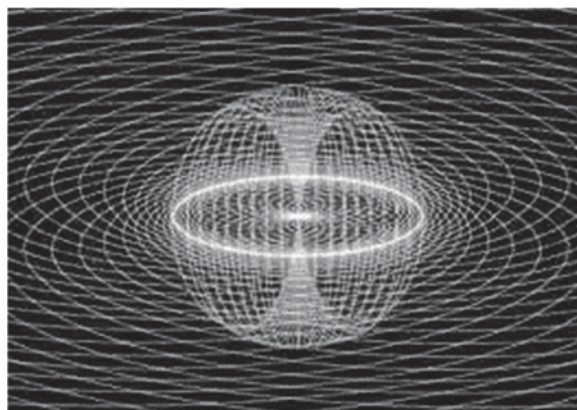
Diagram 2: General depiction of a torus field. Notice the flat plane at the cross section
