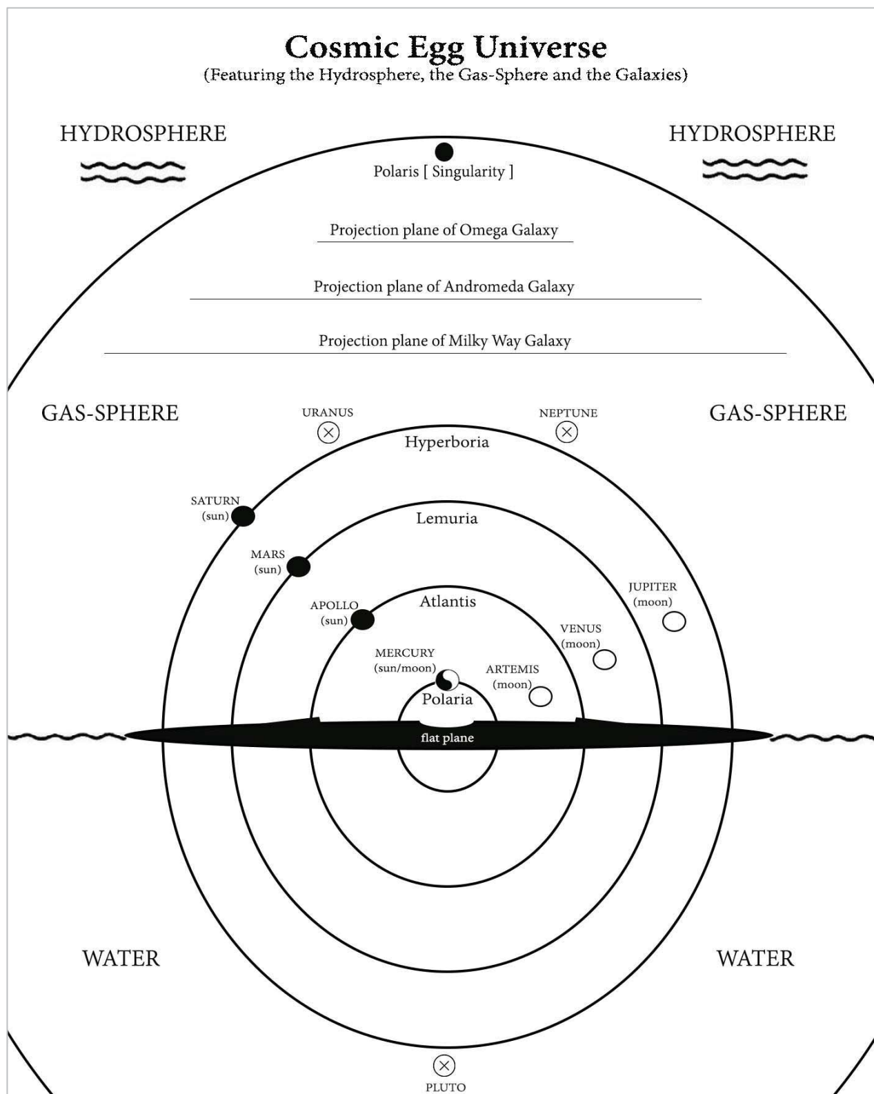
Diagram 9: Cosmic Egg Universe – featuring the Hydrosphere, the Gas-Sphere and the Galaxies.
