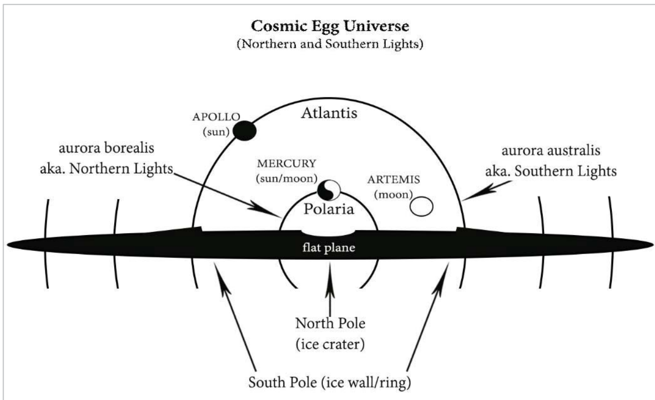
Diagram 6: Northern and Southern Lights – the inner and outer Van Allen belts. These are the two inner most torus fields (that embody the Atlantean and Polarian Realms) of our four dimensional torus field.
