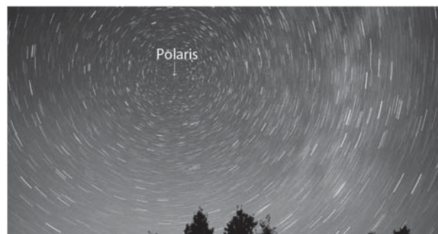
Picture 2: Polaris – North Star or Pole Star
