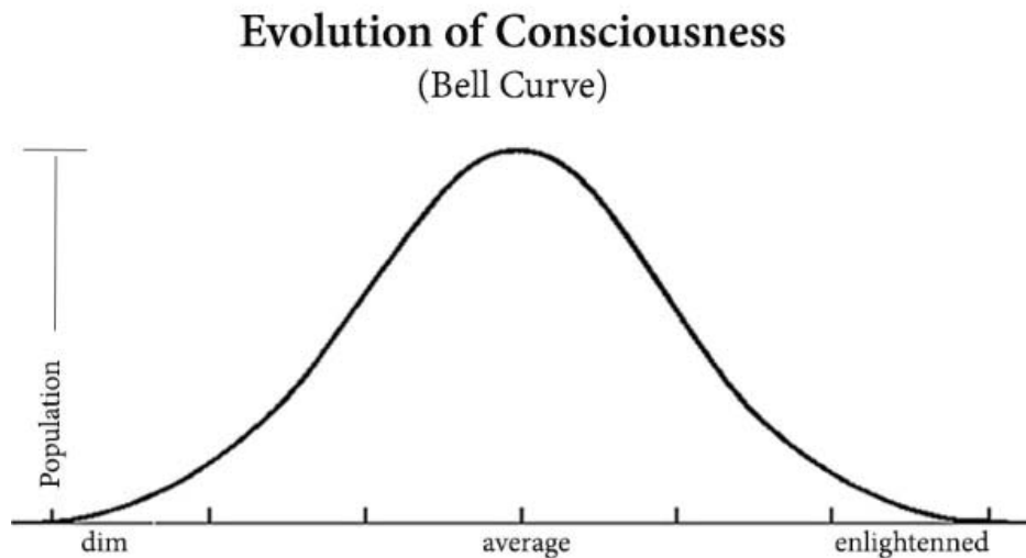
Diagram 4: Bell Curve - Evolution of Consciousness
