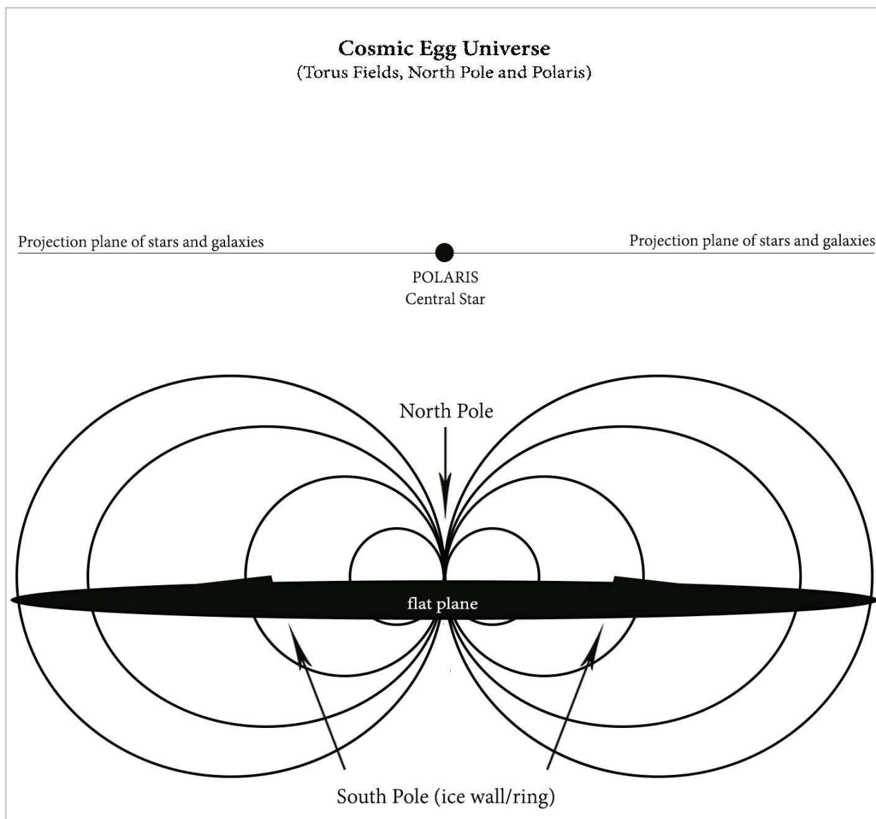
Diagram 5: Torus Fields, North Pole and Polaris
