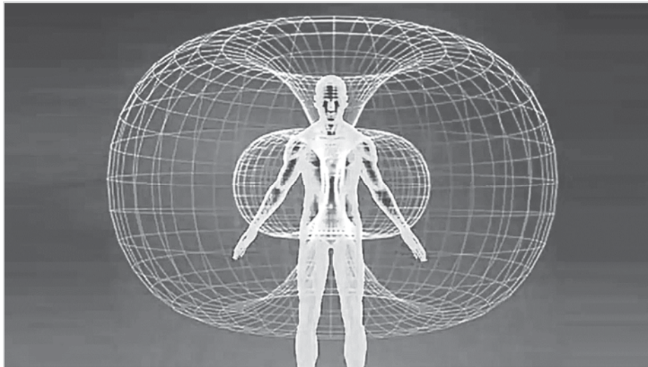
Diagram 3: Torus field radiated from the heart.
