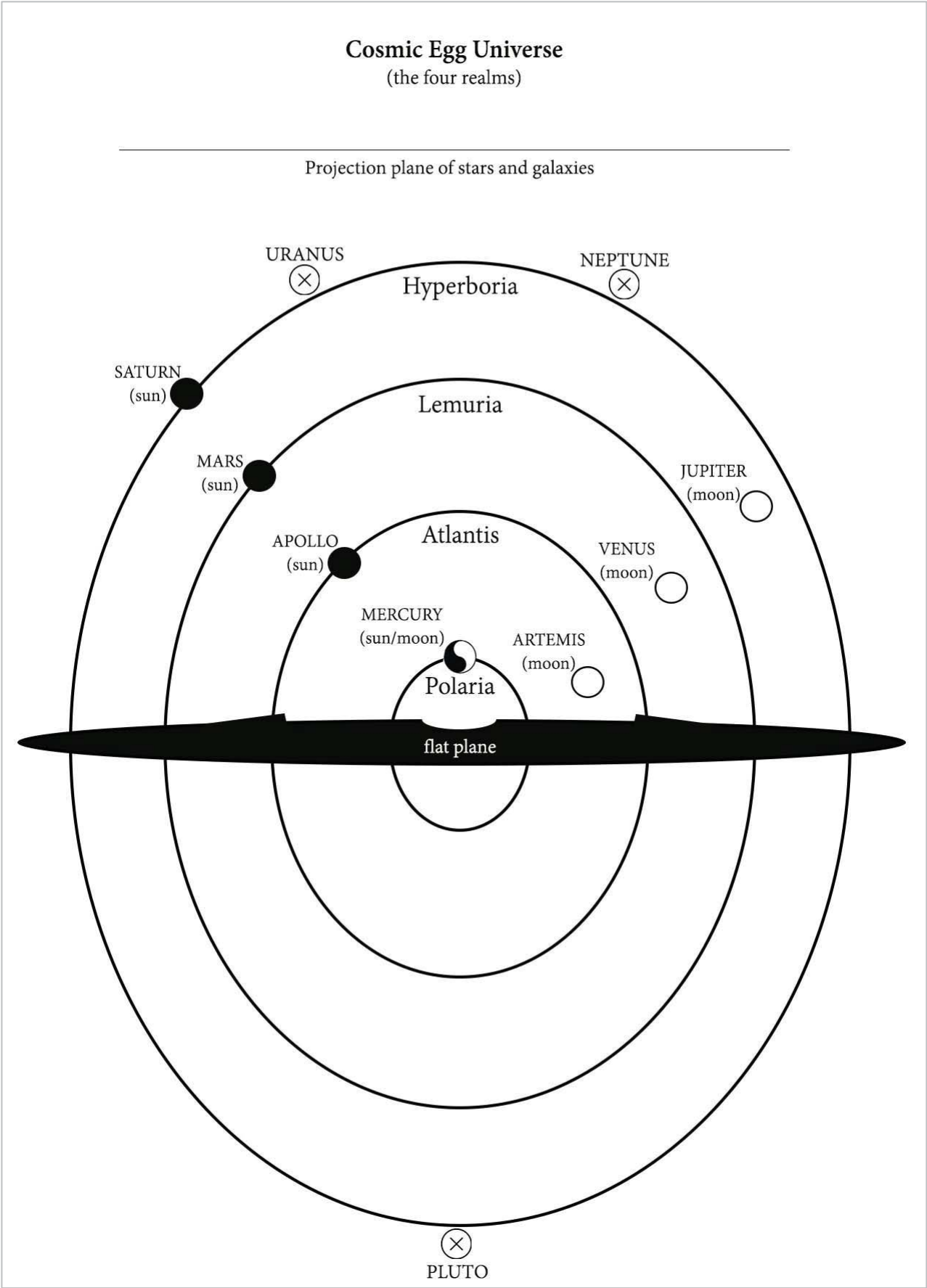
Diagram 8: Martin Kenny’s Cosmic Egg Universe – cross section view
