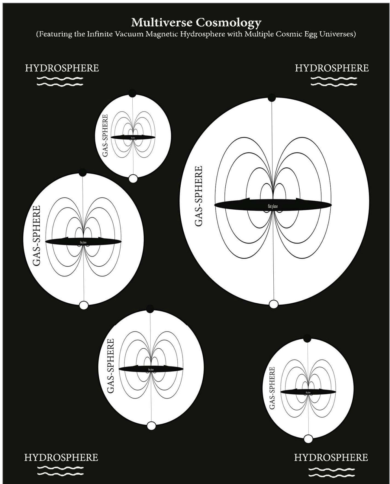
Diagram 10: Depiction of the Multiverse, showing the Infinite Magnetic Hydrosphere Vacuum with multiple Electromagnetic Cosmic Egg Universes inside.
